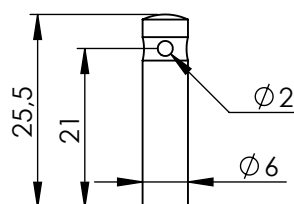
Hohlschraube Threaded busching
