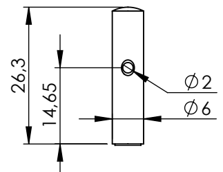
TopLocking 1002XXXX.XX.55
