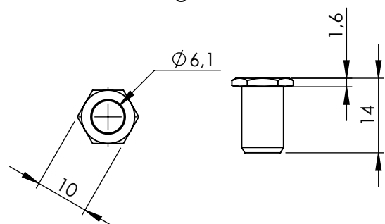
Hohlschraube Threaded busching
