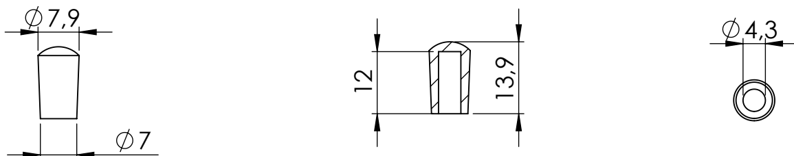
Toggle Switch Knopf toggle switch knob PK: 1521XXXX
