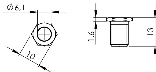
Hohlschraube Threaded bushing
