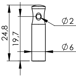
Locking 18,0 1004XXXX.XX.51
