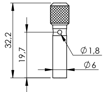
TopLocking 1004XXXX.XX.55
