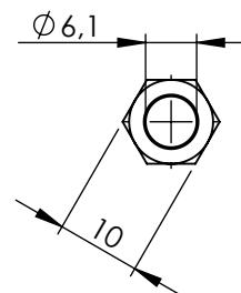
Hohlschraube Threaded bushing
