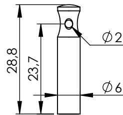
Locking 21,0 1056XXXX.XX.53
