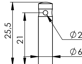
Hohlschraube Threaded bushing
